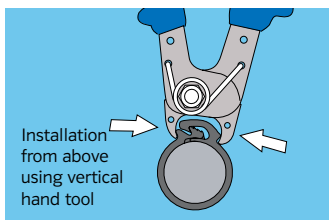
Ezyklik manual and pneumatic installation tools.
